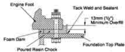
Section A-A Elevation
