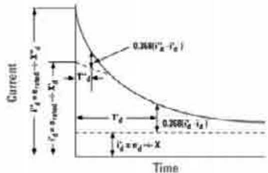
Symmetrical Component of 3-Phase Short Circuit
