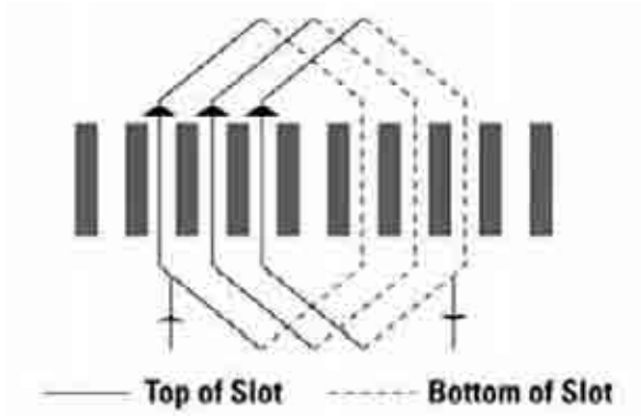
Figure 8. Lap Wound
