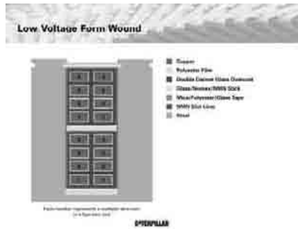
Figure 11. Form Wound
